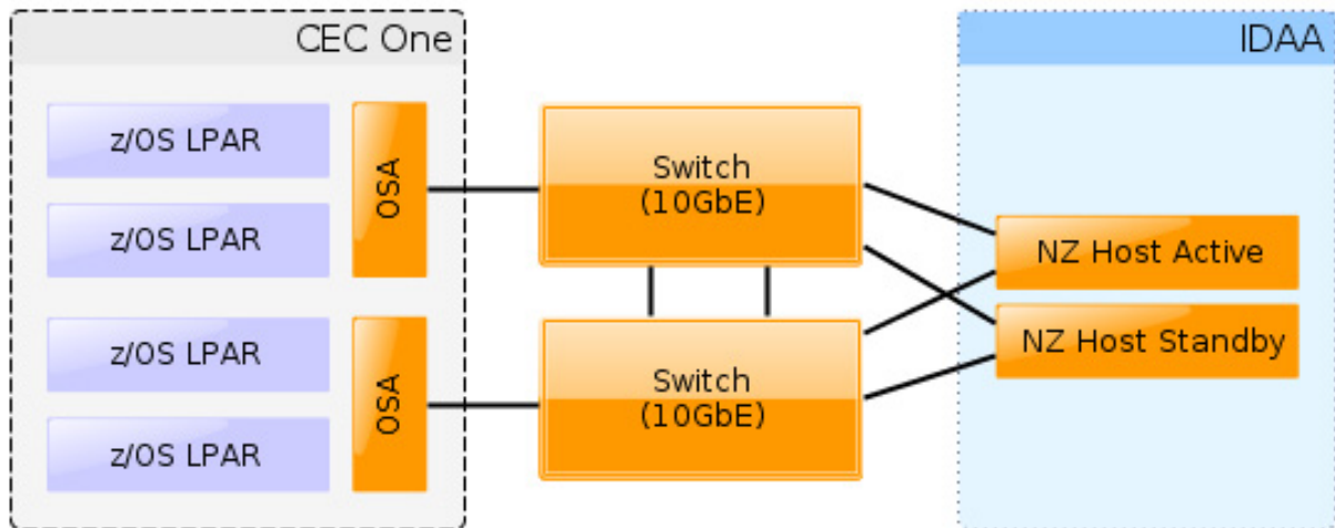
Figure 10. Recommended connections between IBM zEnterprise server and IBM PureData System for Analytics (including switches)
