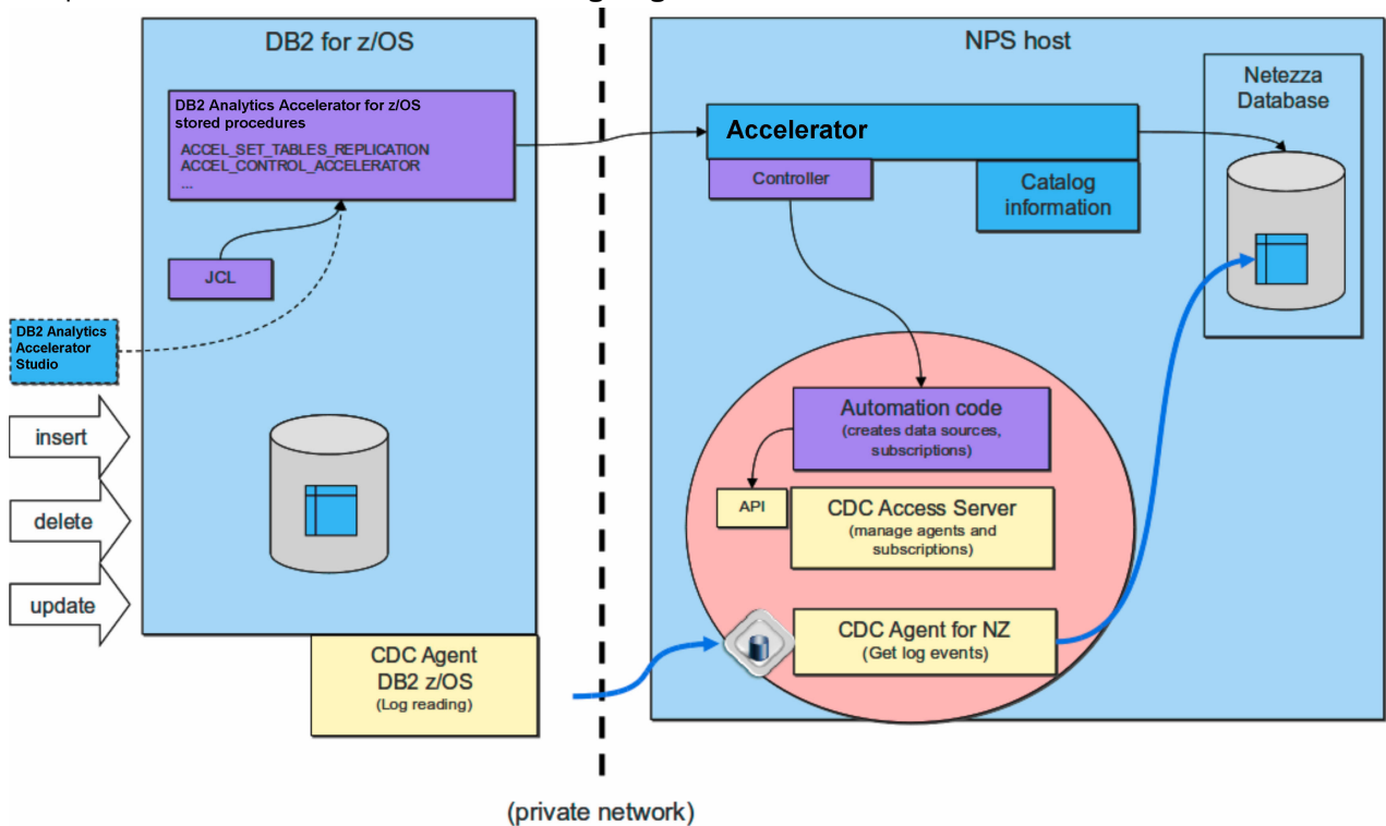
Figure 8. Interaction diagram of the components that are involved in the incremental update process.
