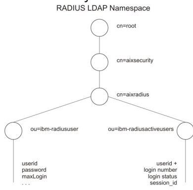
Figure 16. RADIUS LDAP Namespace
