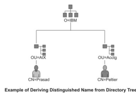
Figure 11. Example of Deriving Distinguished Name from Directory Tree
