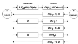
Figure 15. Authentication Process
