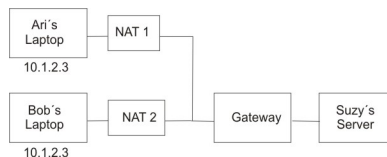
Figure 13. Tunnel Mode Conflict
