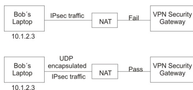
Figure 12. NAT-enabled IP Security
