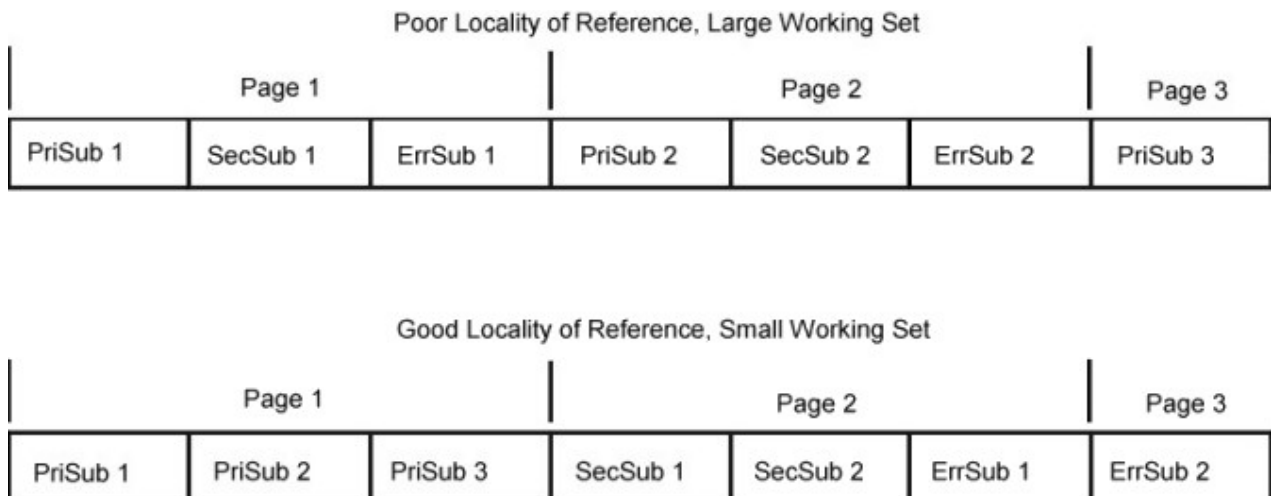
Figure 15. Locality of Reference
