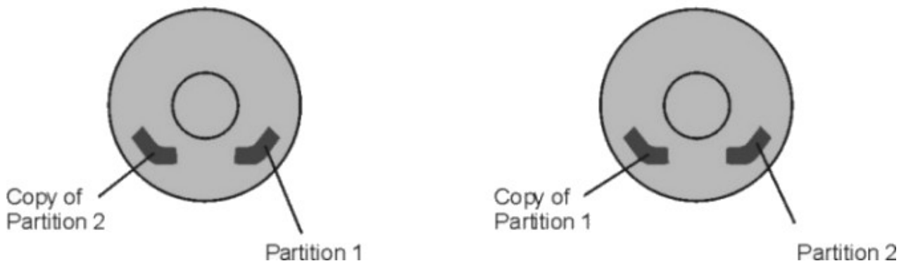
Figure 18. Inter-Physical Volume Allocation Policy
