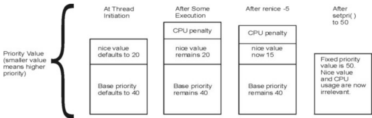
Figure 6. How the Priority Value is Determined
