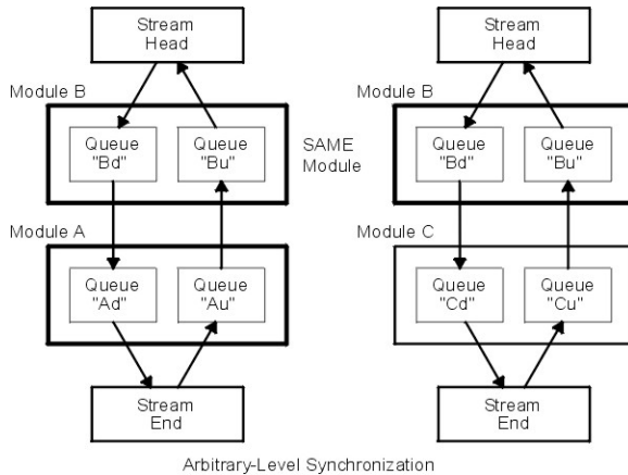
Figure 38. Arbitrary-Level Synchronization
