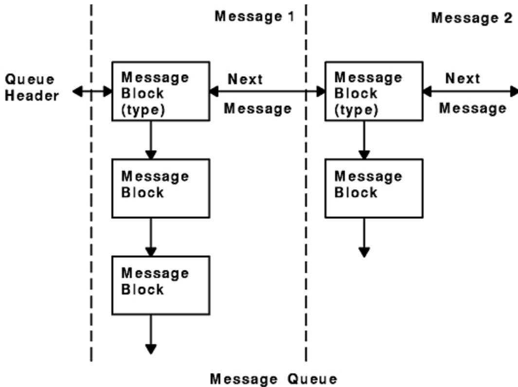
Figure 43. Message Queue
