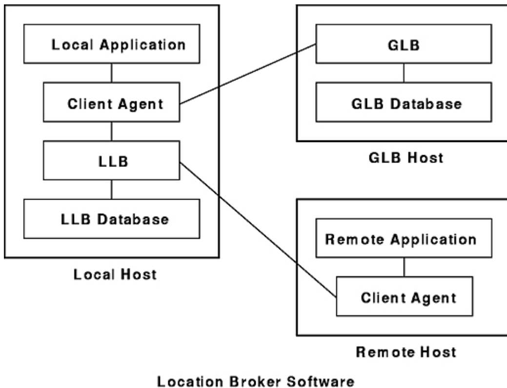
Figure 21. Location Broker Software
