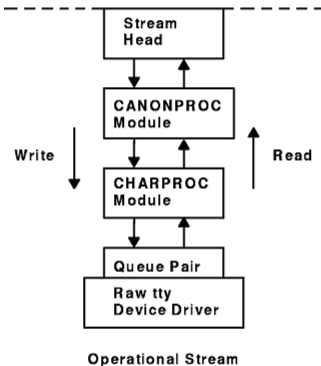
Figure 47. Operational Stream
