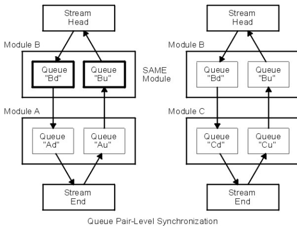
Figure 36. Queue Pair-Level Synchronization
