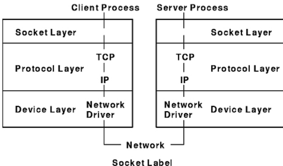
Figure 29. Socket Label
