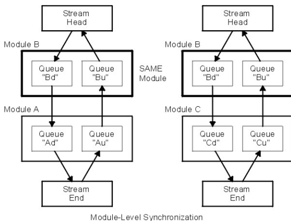
Figure 37. Module-Level Synchronization
