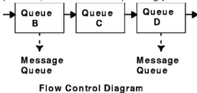
Figure 34. Flow Control
