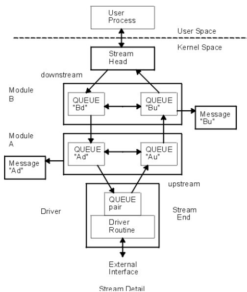
Figure 32. Stream Detail
