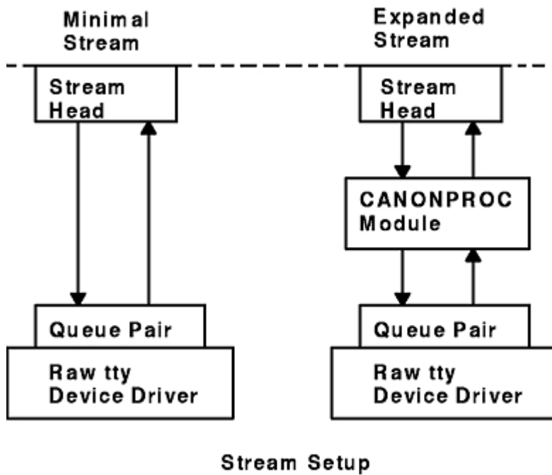
Figure 41. Stream Setup
