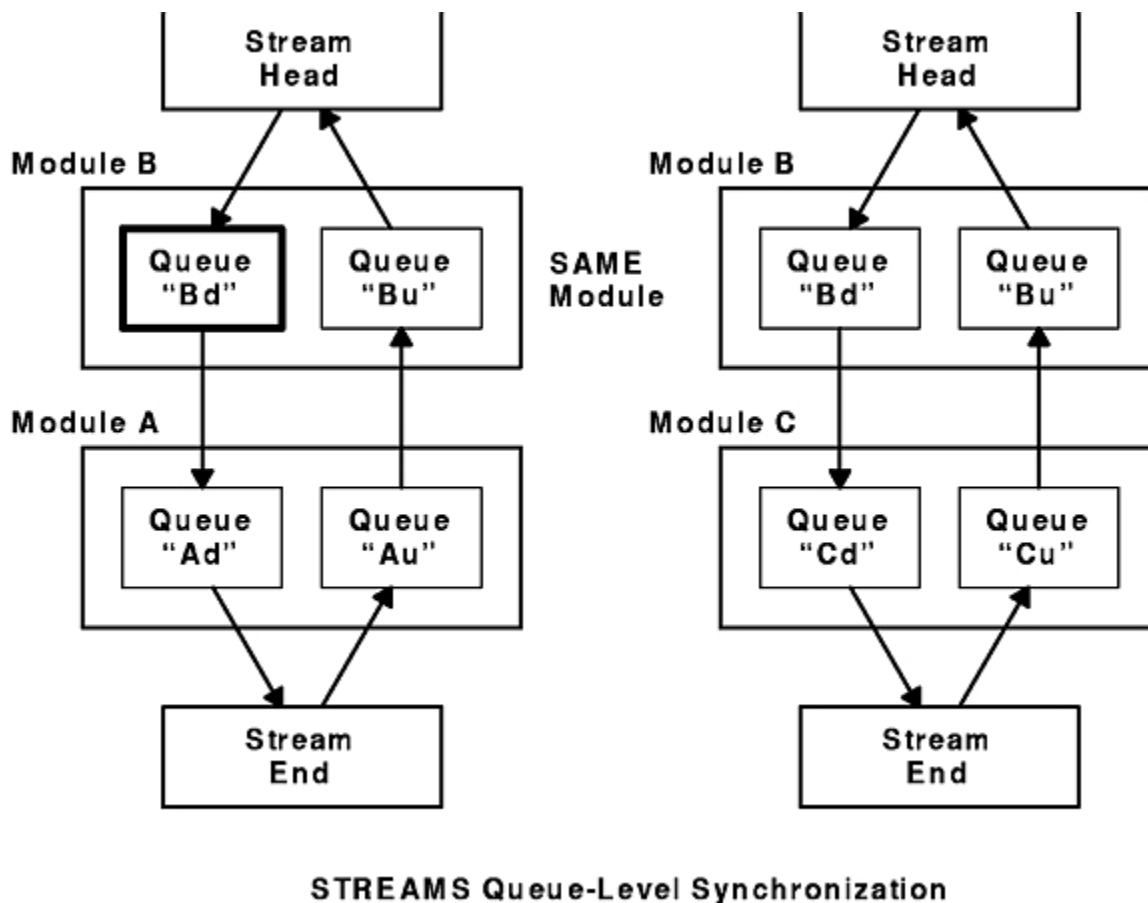
Figure 35. STREAMS Queue-Level Synchronization
