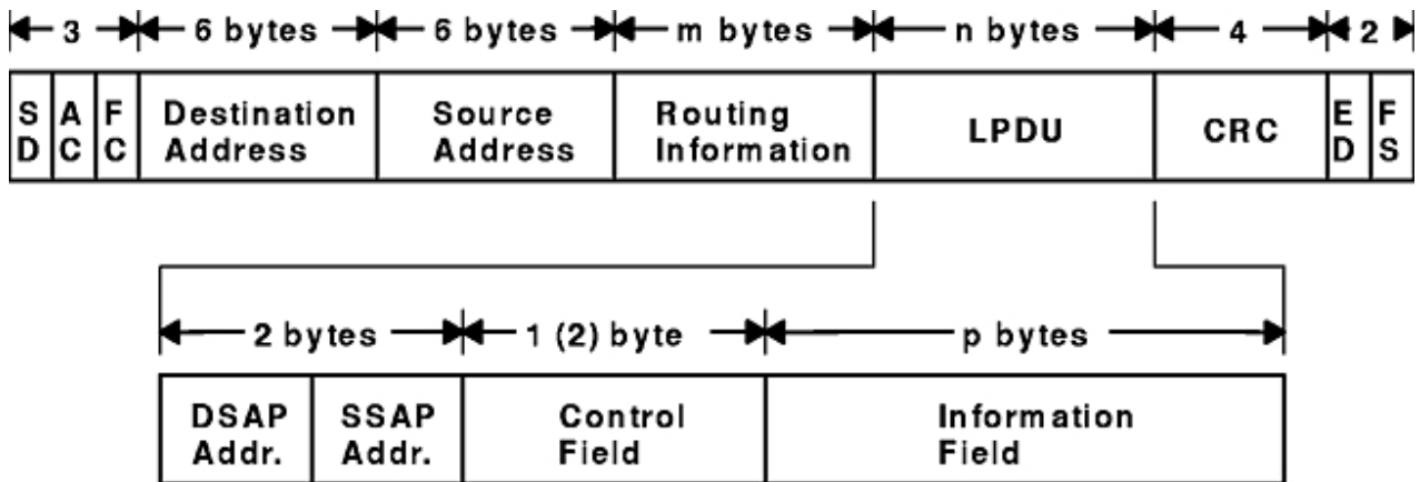
DLCTOKEN Frame Encapsulation
