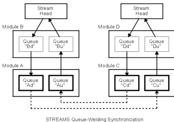
Figure 39. STREAMS Queue-Welding Synchronization
