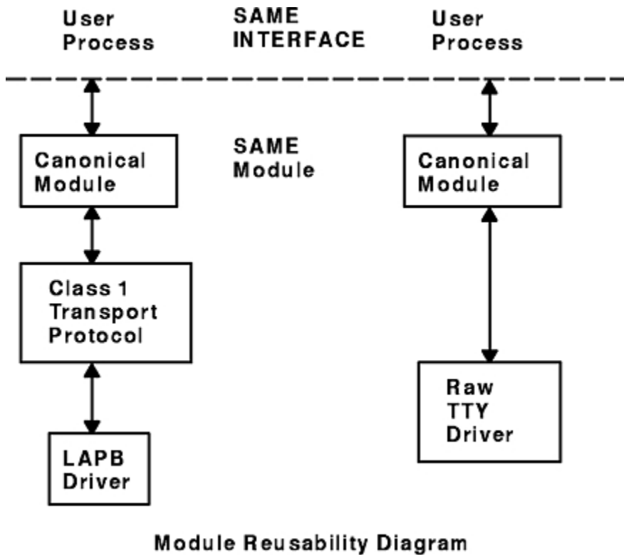
Figure 33. Module Reusability Diagram
