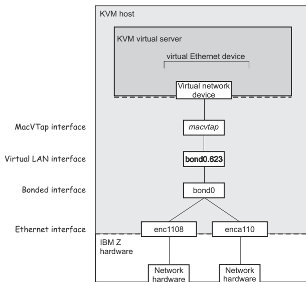
Figure 21. Direct interface type which configures a virtual LAN interface
