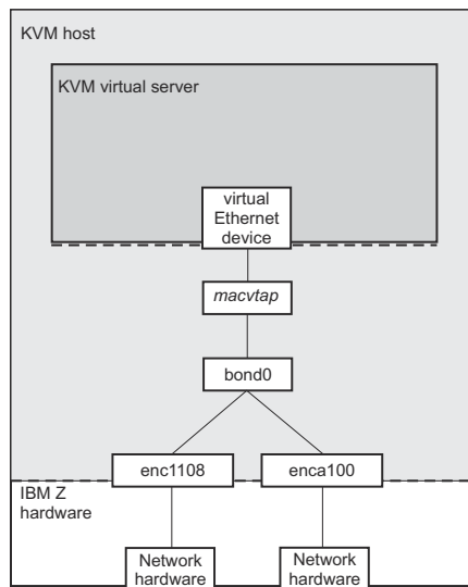
Figure 20. Direct interface type which configures a bonded interface
