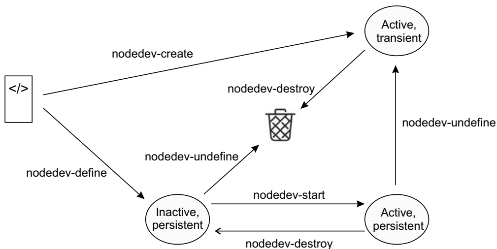
Figure 19. Lifecycle of VFIO mediated devices and virsh nodedev commands
