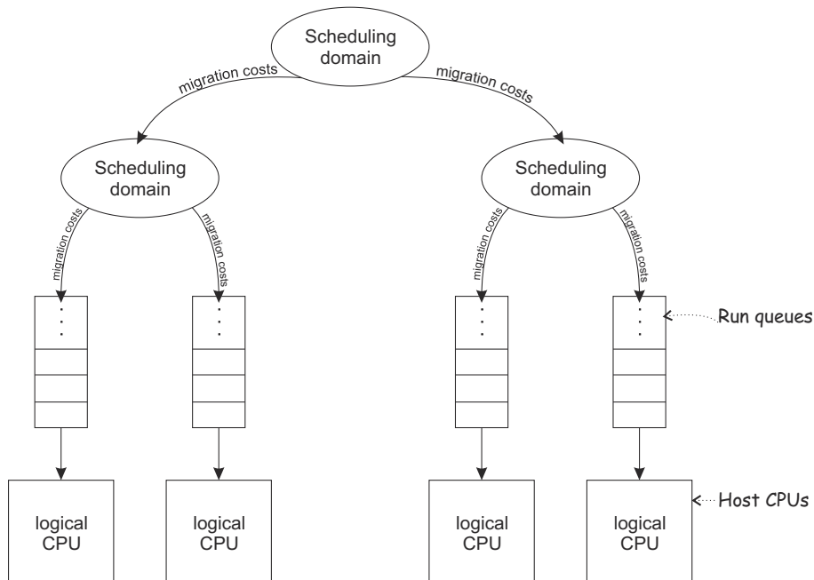
Figure 26. Linux scheduling
