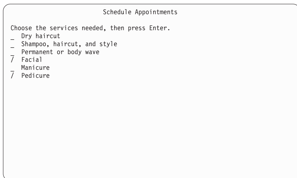
Figure 35. Multiple-choice selection field
