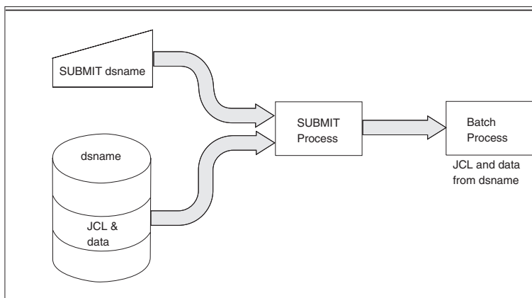
Figure 7. The SUBMIT Process With User-Created JCL Statements
