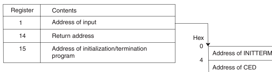
Figure 8. Registers Passed at Initialization
