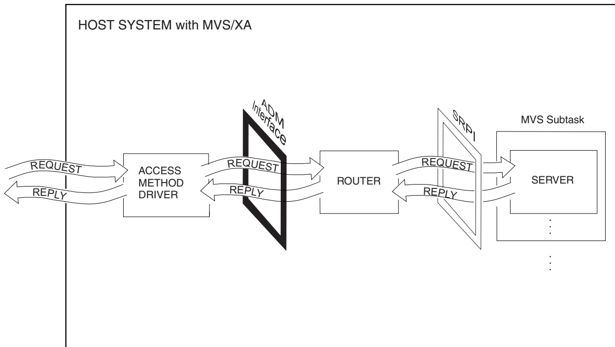
Figure 11. The MVSSERV Enhanced Connectivity Environment
