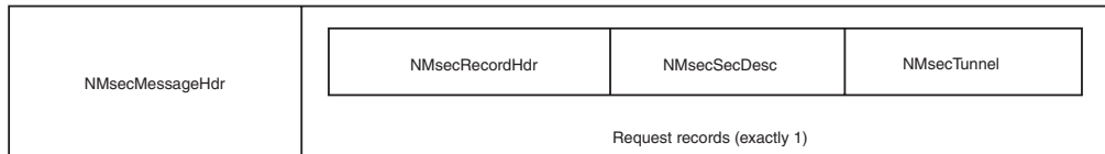
Figure 17. NMsec_REFRESH_IKETUN request format
