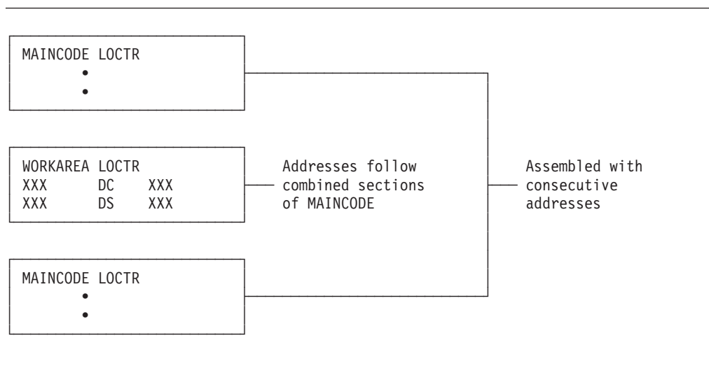
Figure 1. LOCTR instruction application
