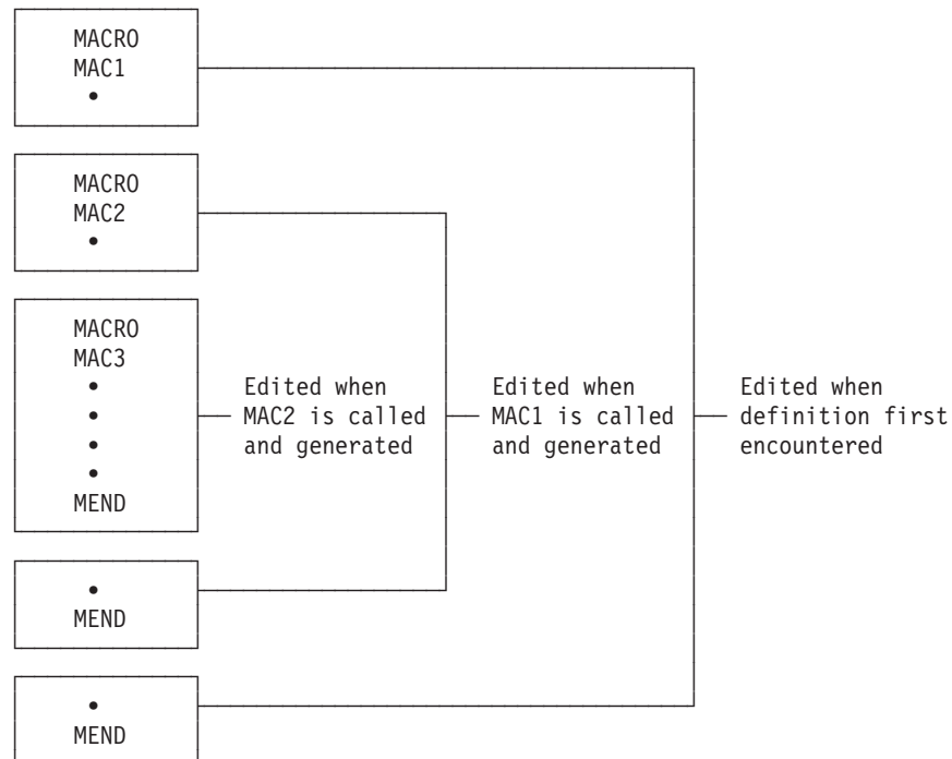
Figure 2. Editing inner macro definitions
