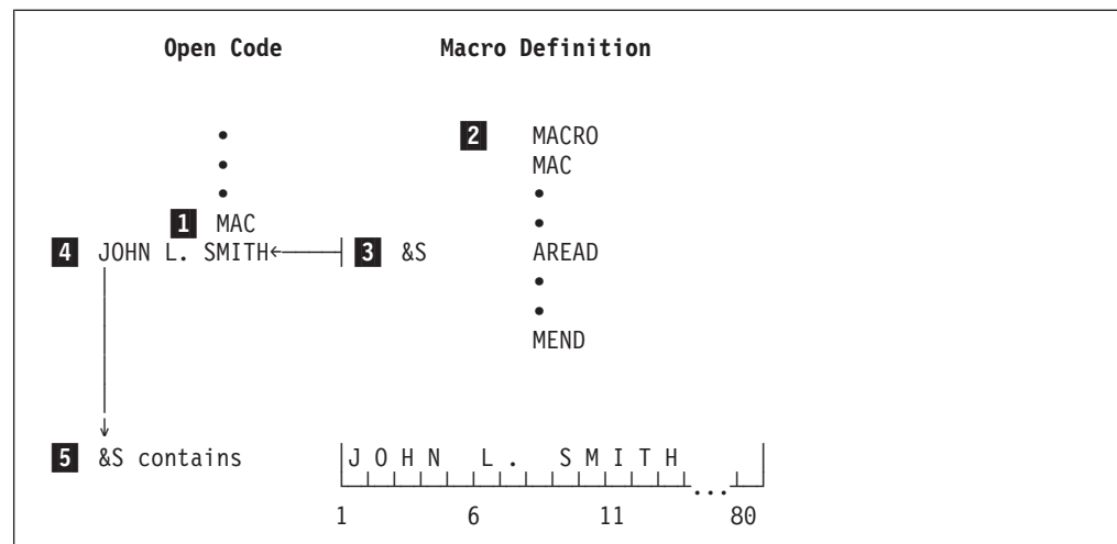
Figure 3. AREAD assembler operation
