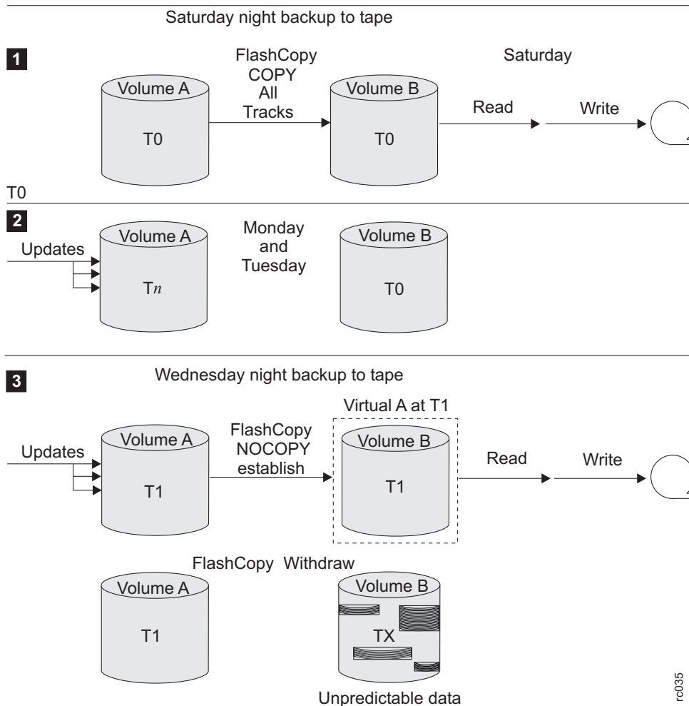
Figure 56. The state of a target volume after a FCWITHDR command processes
