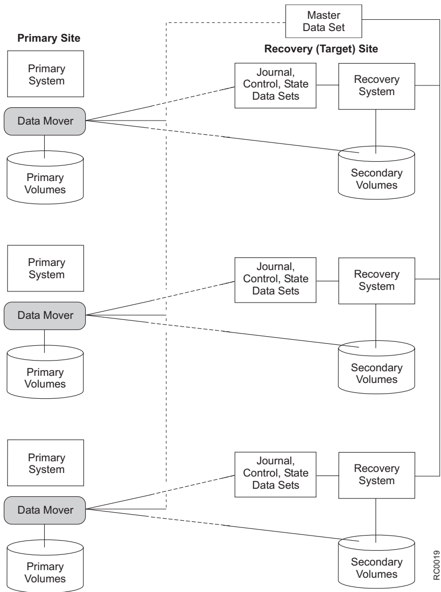
Figure 7. CXRC configuration with system data mover at primary site
