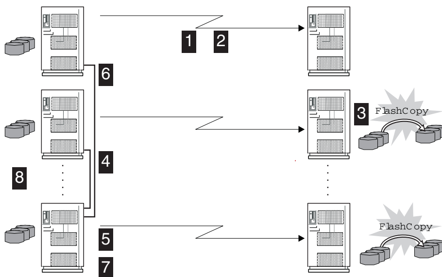
Figure 37. Setting Up Global Mirror for ESS
