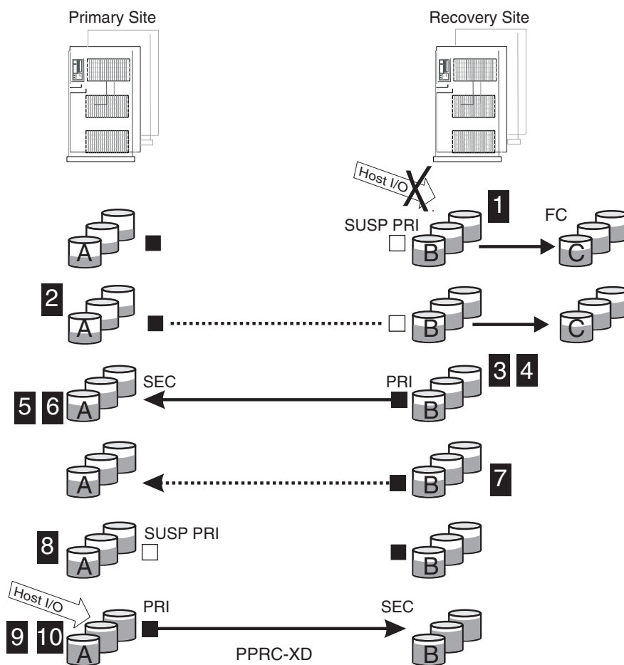
Figure 29. Failback in a PPRC-XD Environment
