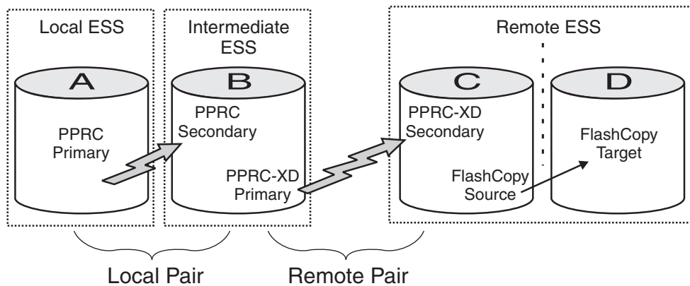
Figure 13. Metro/Global Copy with optional FlashCopy
