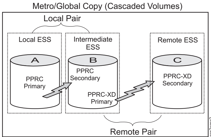
Figure 20. Metro/Global Copy (Cascaded Volumes)
