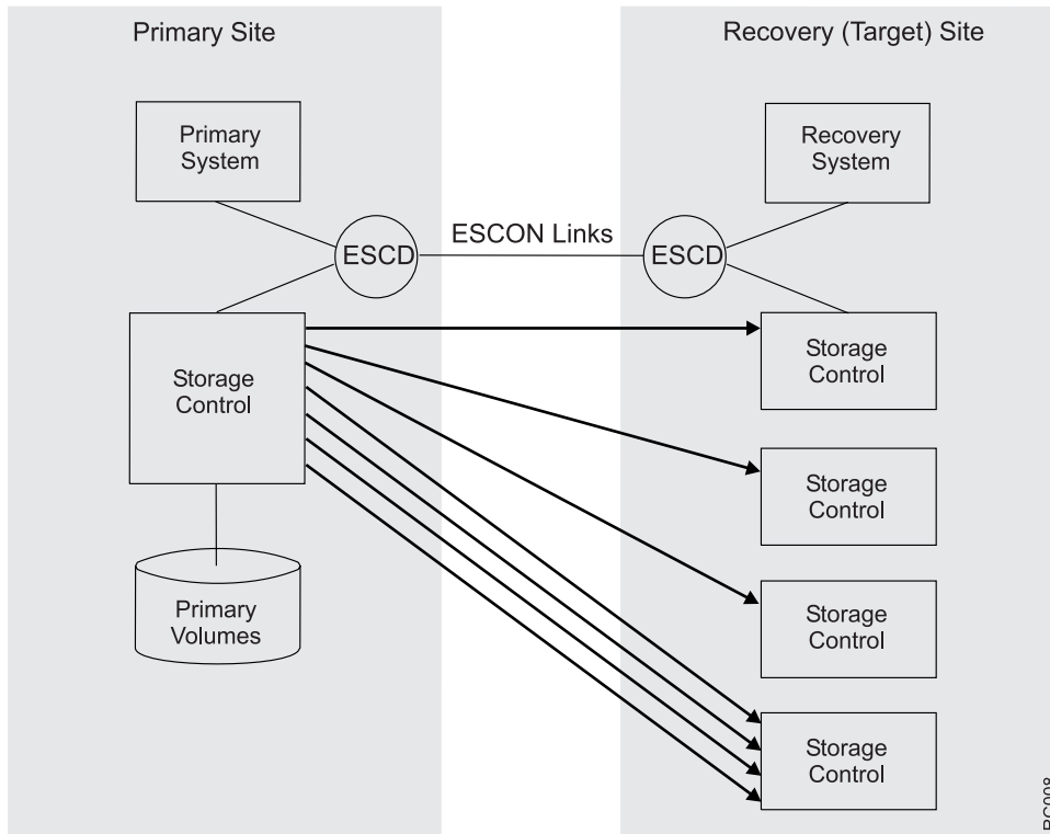
Figure 11. PPRC ESCON path options
