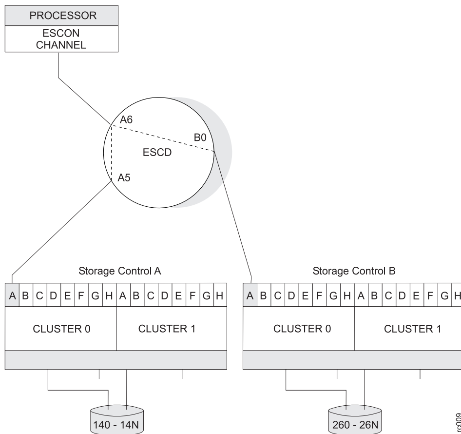
Figure 22. Storage subsystems for primary and secondary volumes
