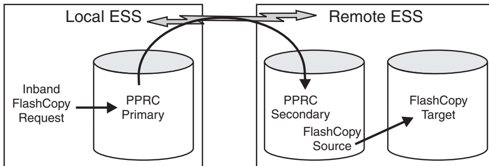
Figure 50. Inband FlashCopy Requests Are Transmitted from PPRC Primary to PPRC Secondary
