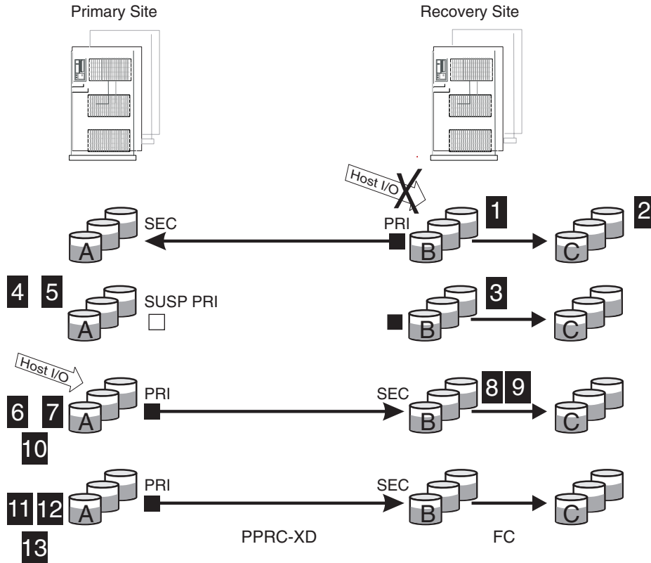
Figure 45. Returning Global Mirror to Primary Site in an Unplanned Outage
