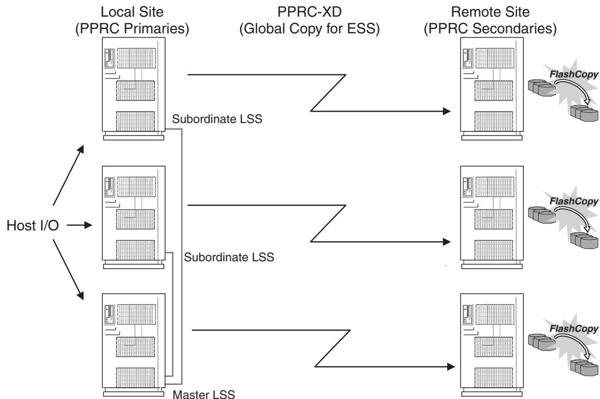
Figure 36. Global Mirror for ESS Combines PPRC-XD Pair with FlashCopy
