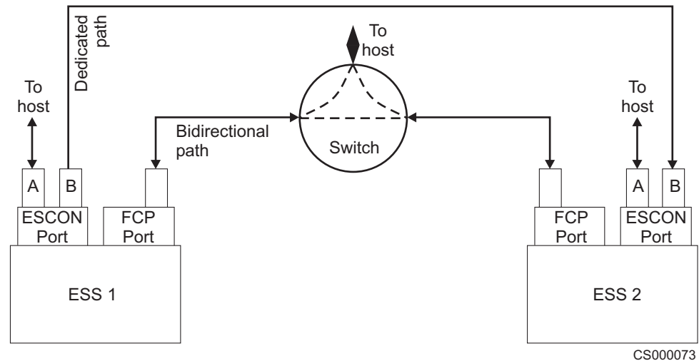
Figure 12. ESCON and FCP configuration
