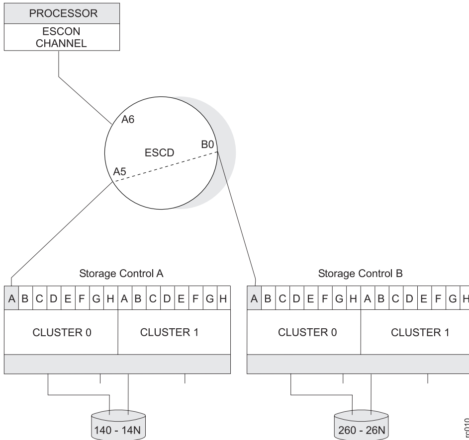
Figure 23. Establishing a PPRC path through an ESCD
