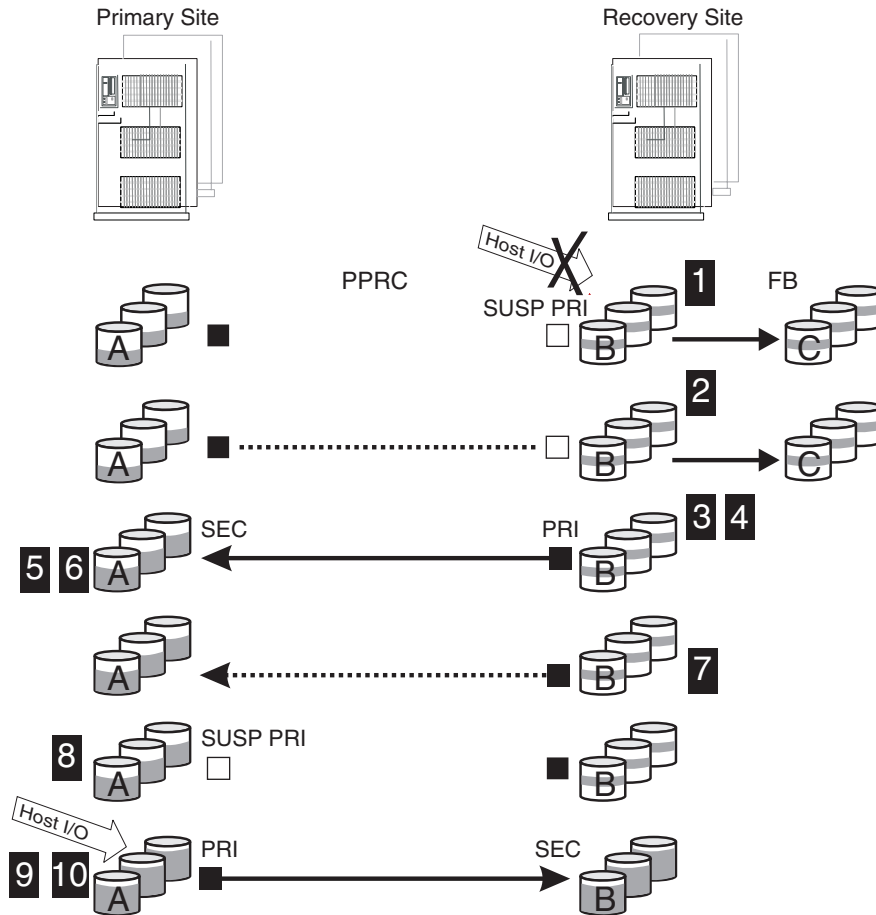
Figure 27. Failback in a Synchronous PPRC Environment
