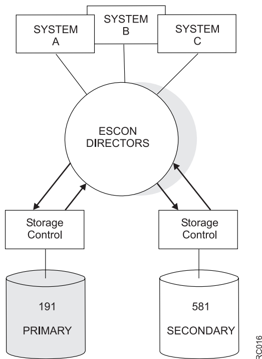
Figure 34. A typical PPRC configuration before a P/DAS operation. Disk device 191 is the PPRC primary volume, receiving updates from three attached systems, A, B and C, through a network of ESCON Directors. PPRC copies all updates to secondary volume 581.
