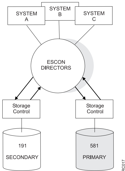
Figure 35. P/DAS swap operation complete. Disk device 581 is now the PPRC primary volume, receiving updates from attached systems through a network of ESCON Directors. PPRC copies all updates to device 191, which has now become the secondary volume.
