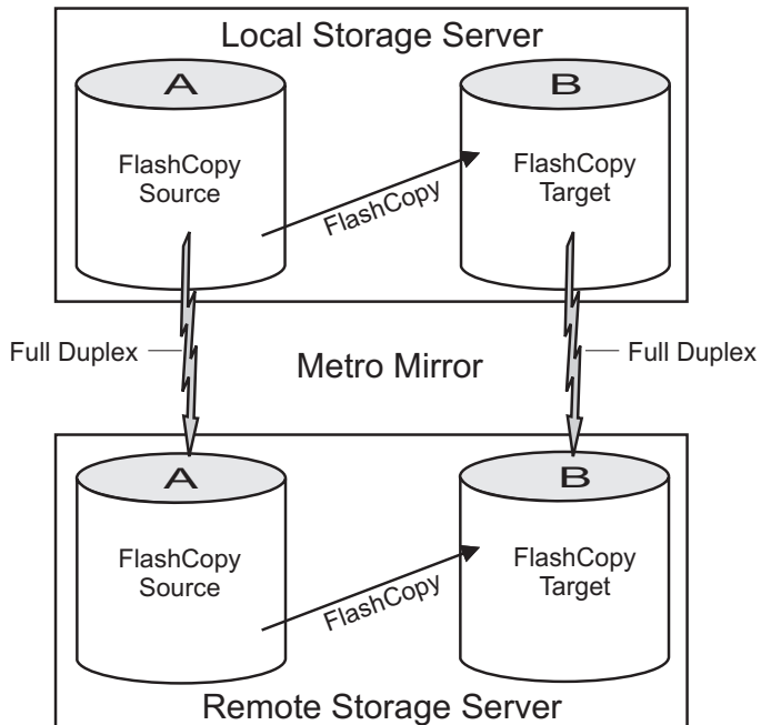
Figure 55. FlashCopy Target as PPRC Primary with Preserve Mirroring
