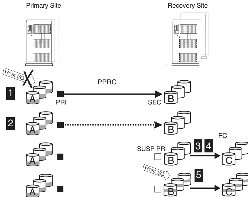
Figure 26. Failover in a Synchronous PPRC Environment
