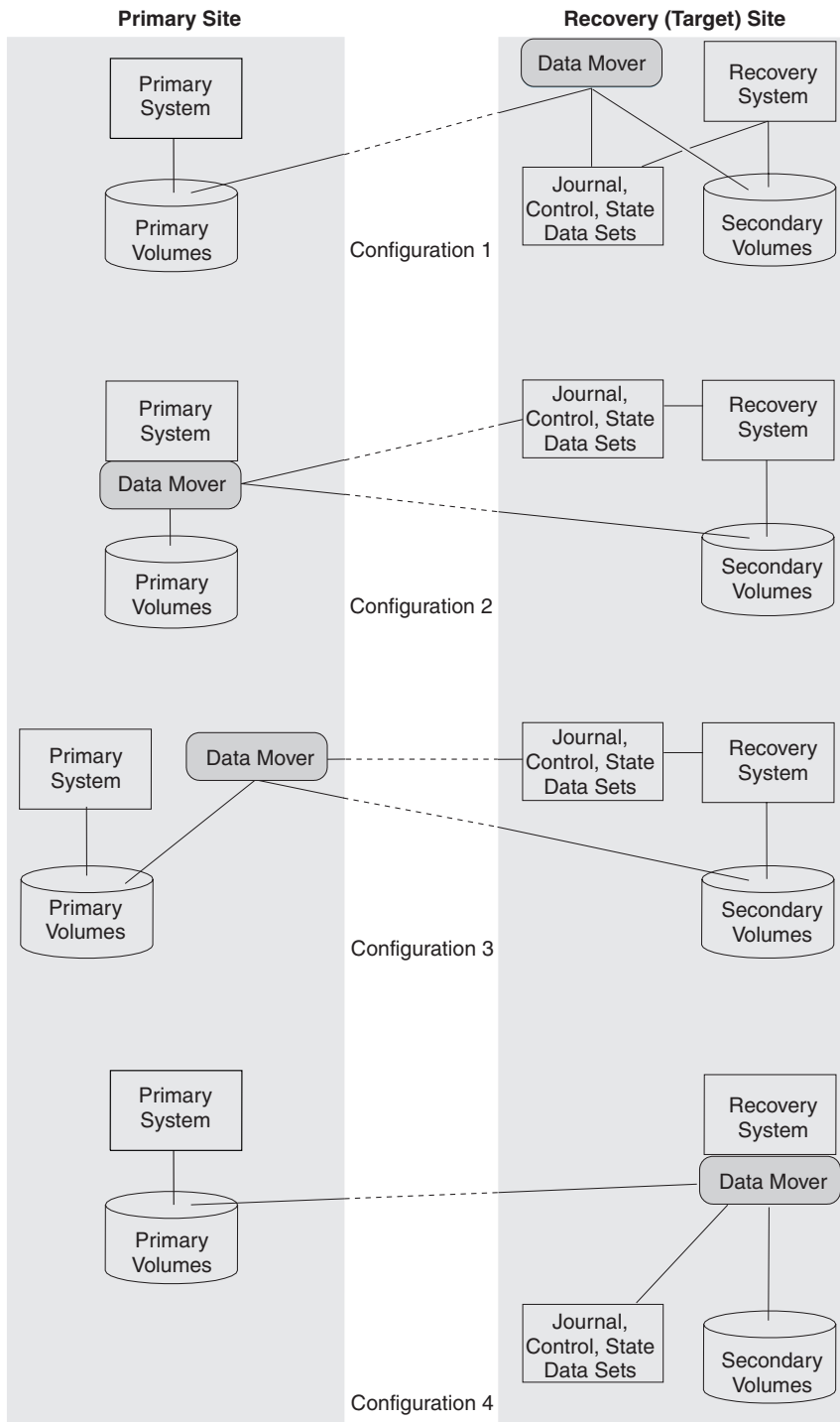
Figure 5. Basic XRC configurations
