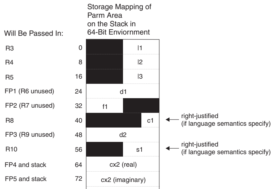
Figure 9. Storage mapping of parm area on the stack in 64-bit environment
