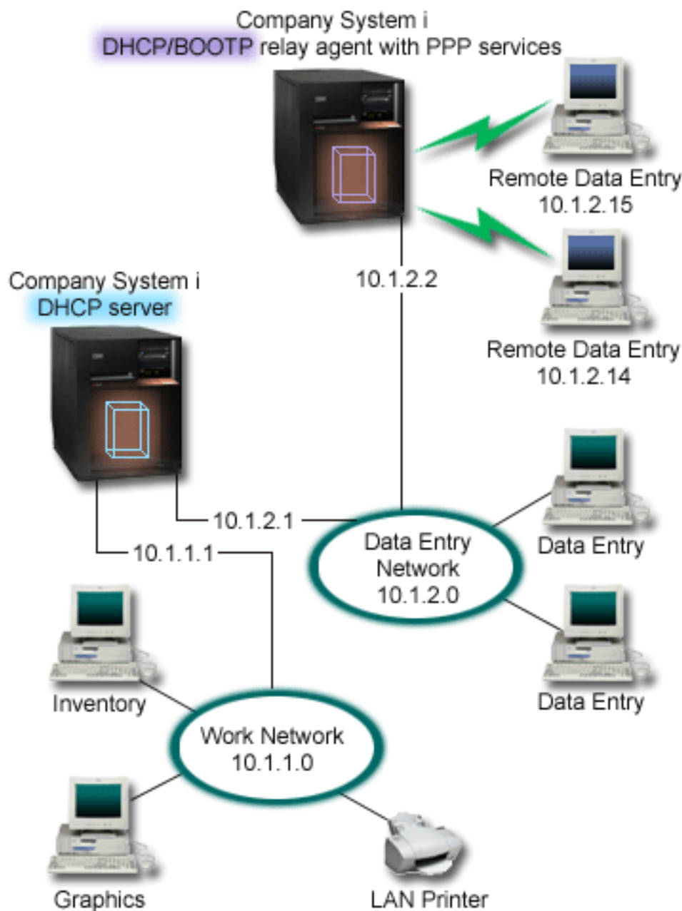
Figure 9. DHCP and PPP profile on different IBM i models
