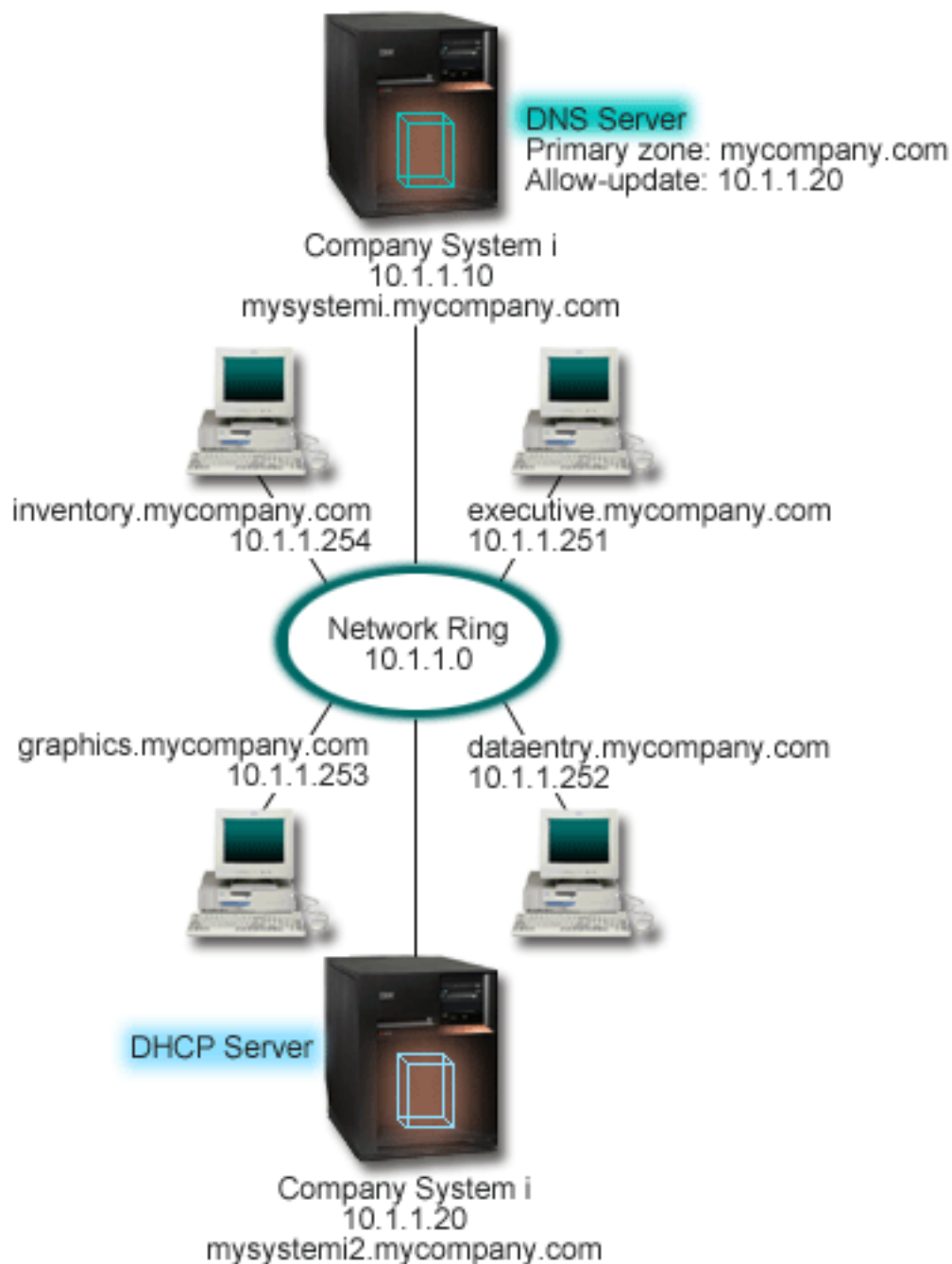
Figure 7. DNS and DHCP on different IBM i models
