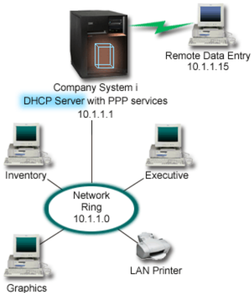
Figure 8. PPP and DHCP on a single IBM i model
