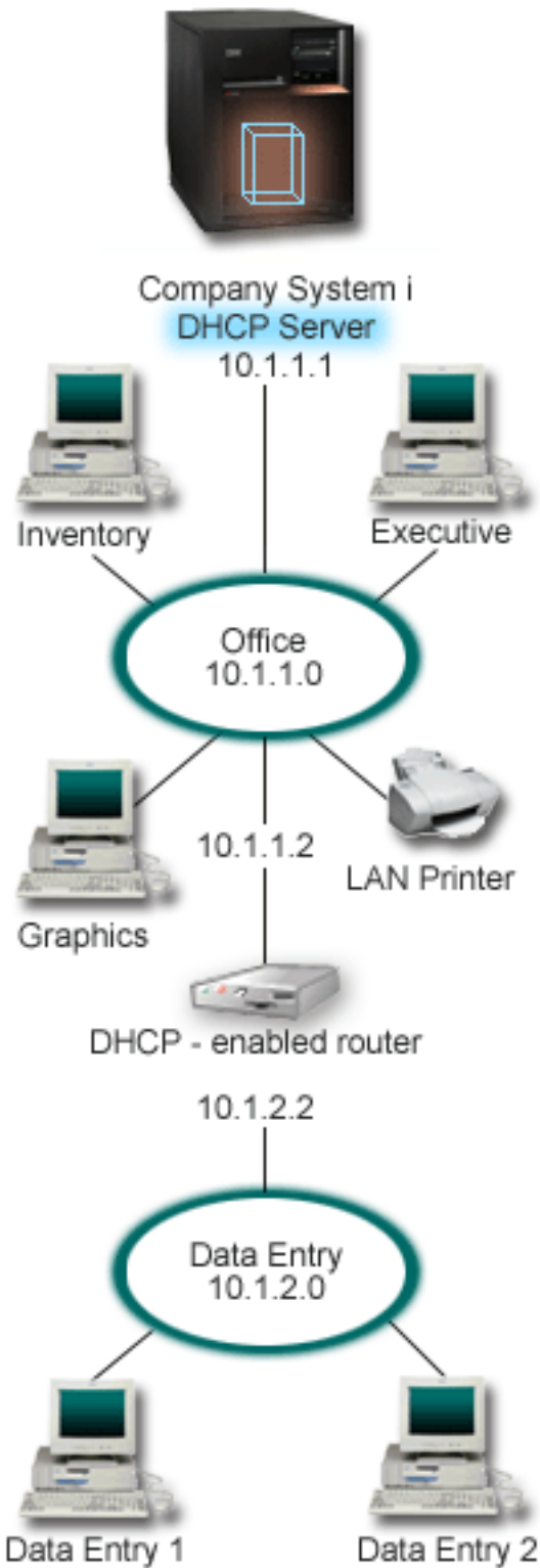
Figure 3. Multiple LANs connected through a router
