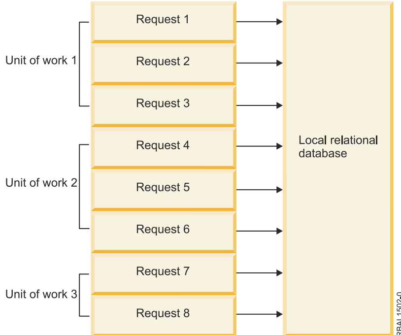
Figure 3. Unit of work in a local relational database
