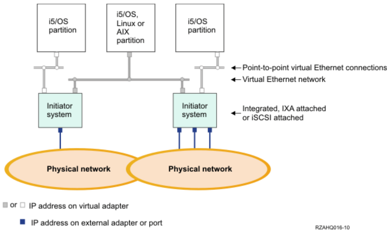
Figure 9. A simple, inter-partition virtual Ethernet network
