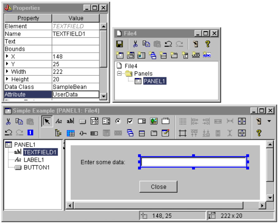
Figure 4: GUI Builder windows: Setting the Attribute property
