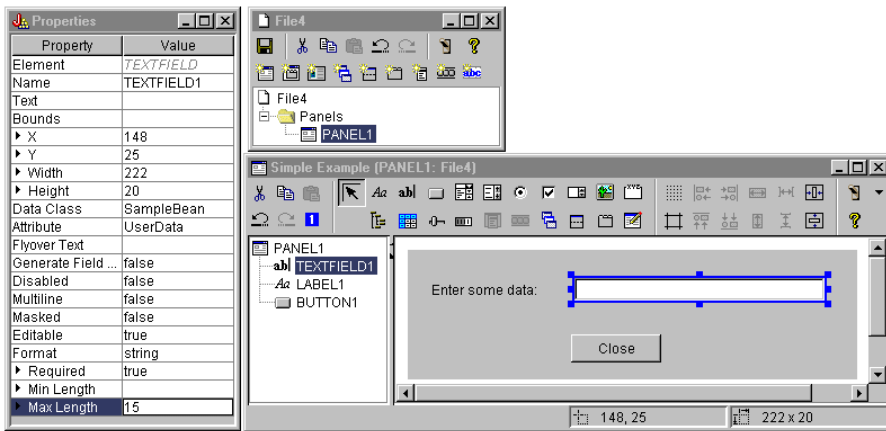
Figure 5: GUI Builder windows: Setting the maximum length of the text field
