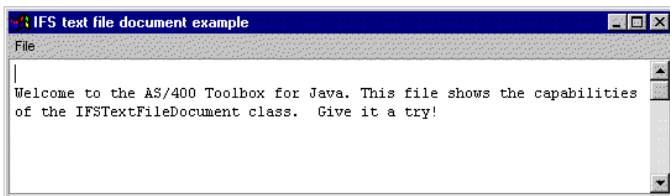
Figure 1: IFSTextFileDocument example
