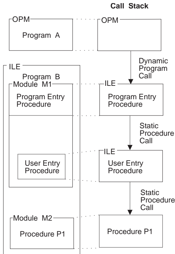
Figure 40. Dynamic Program Calls and Static Procedure Calls on the Call Stack
