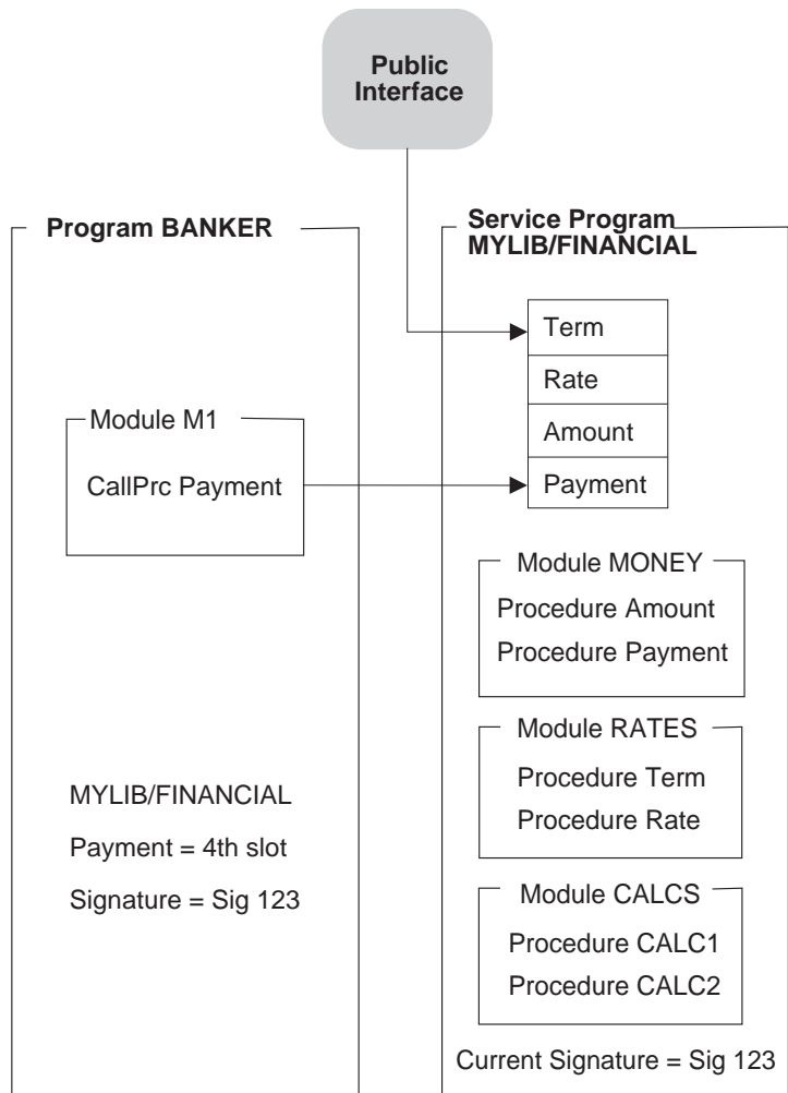
Figure 34. Using the Service Program FINANCIAL
