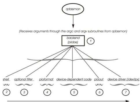
Figure 2. Datastream Flow for Common Print Jobs
