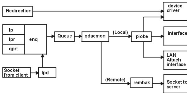
Figure 1. Printing with the Base Operating System
