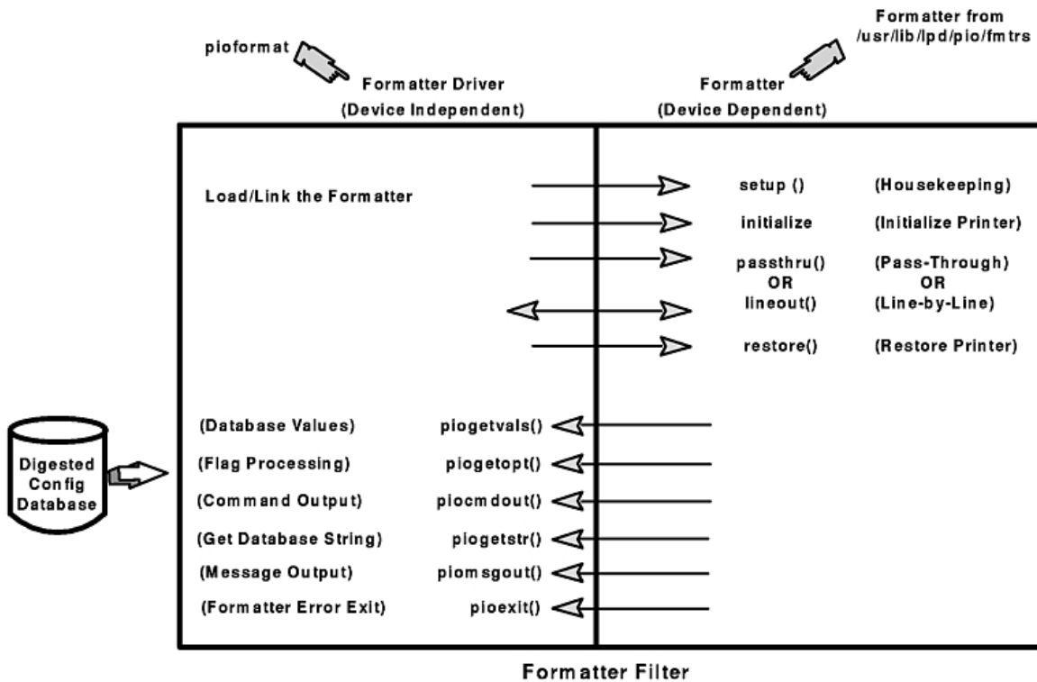
Figure 3. The Formatter Filter
