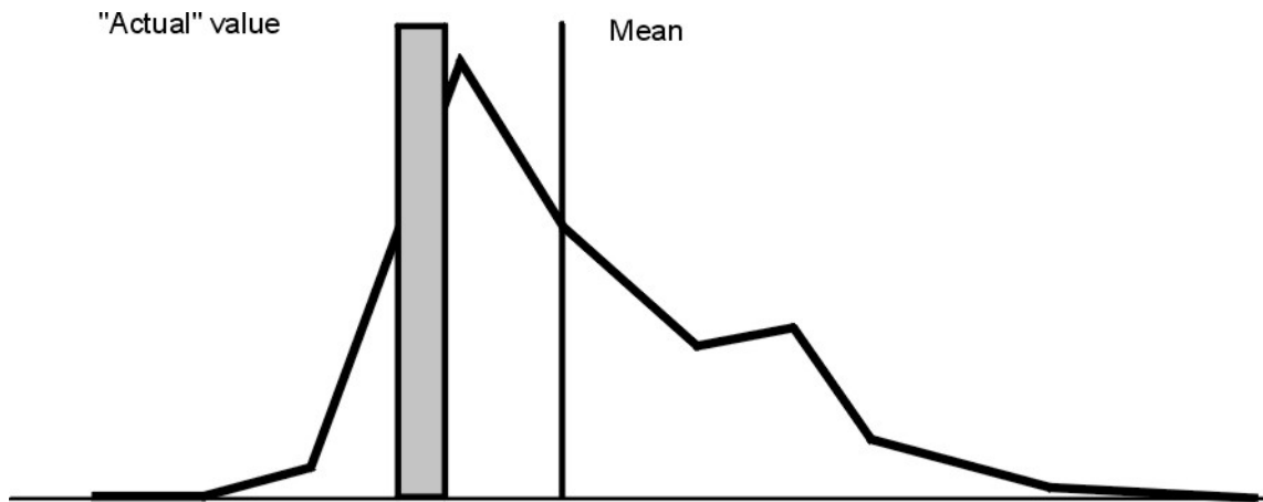
Figure 4. Bimodal Curve
