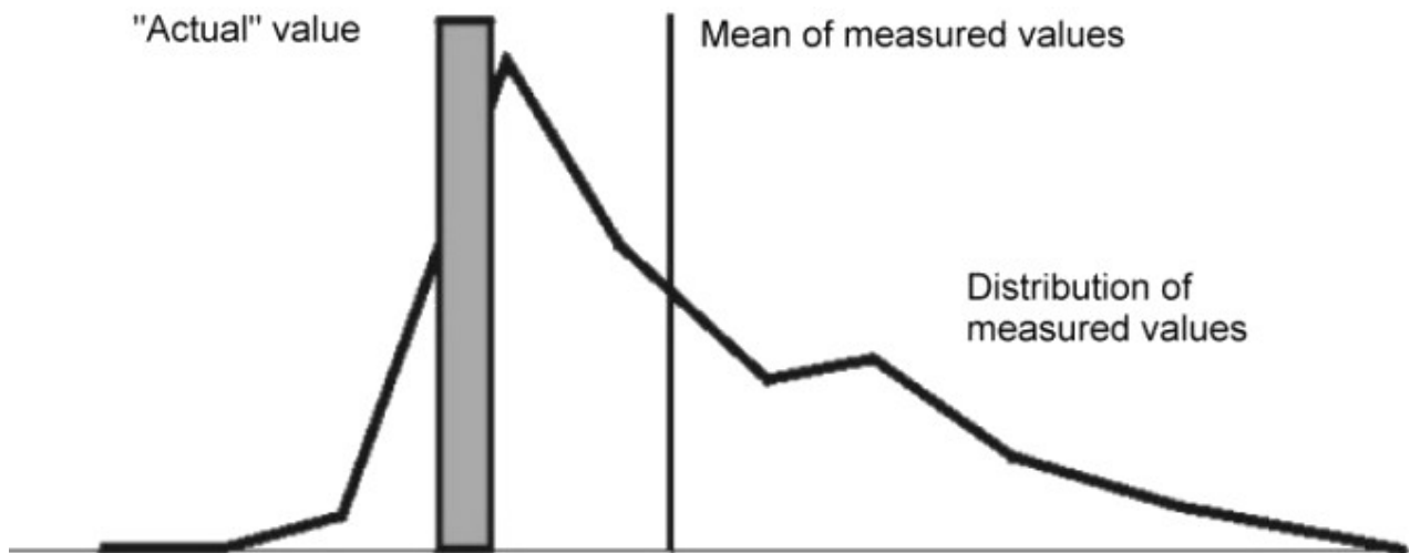
Figure 5. Skewed Curve
