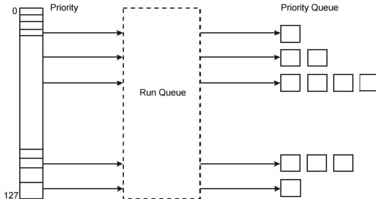
Figure 7. Run Queue
