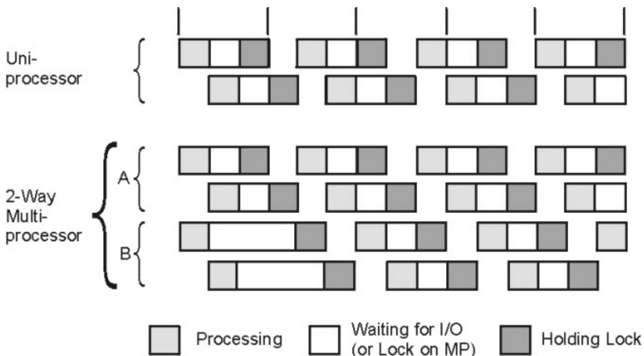
Figure 13. Multiprocessor Scaling
