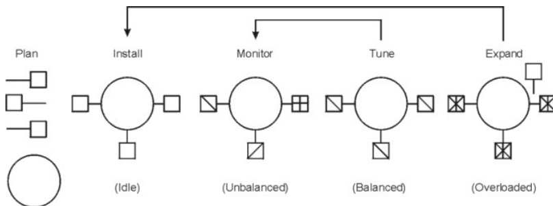
Figure 2. Performance Phases
