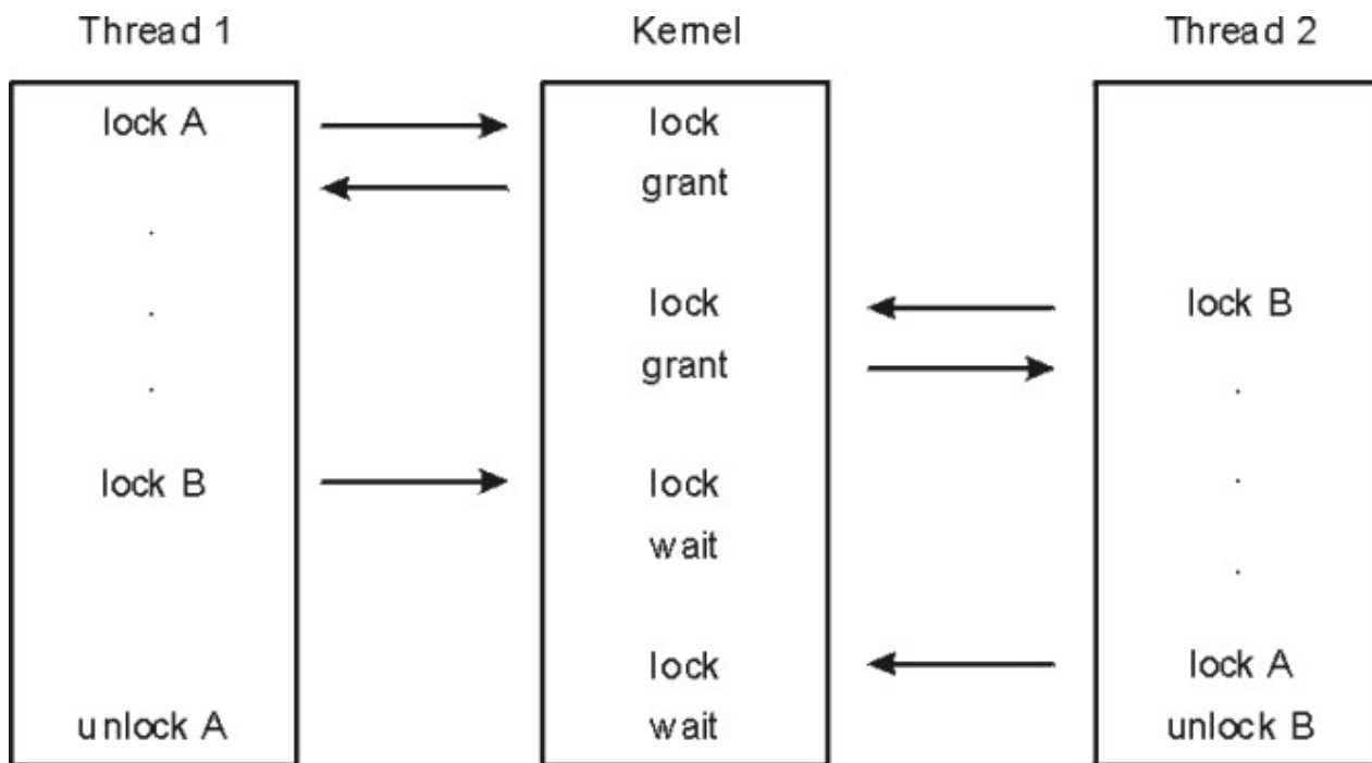
Figure 11. Deadlock
