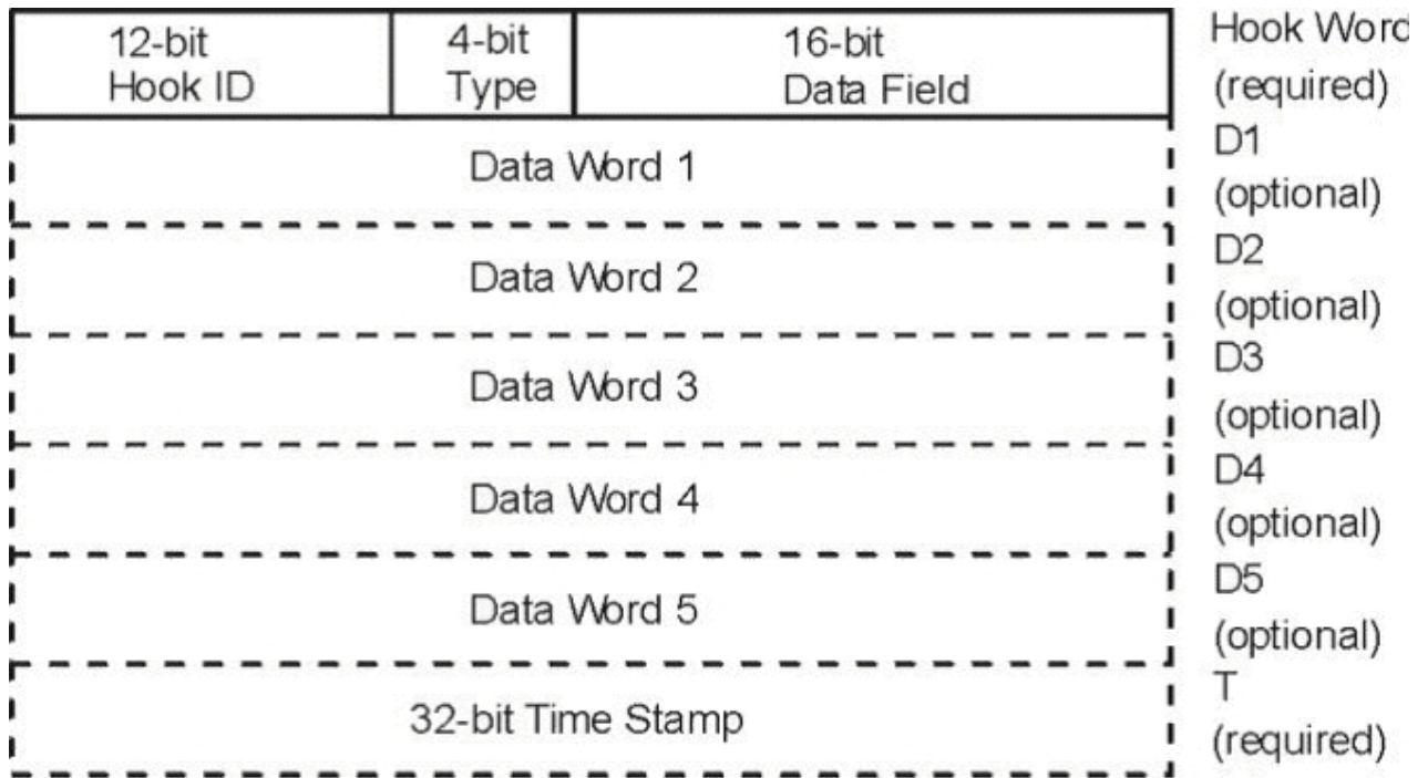
Figure 26. Format of a Trace Event Record
