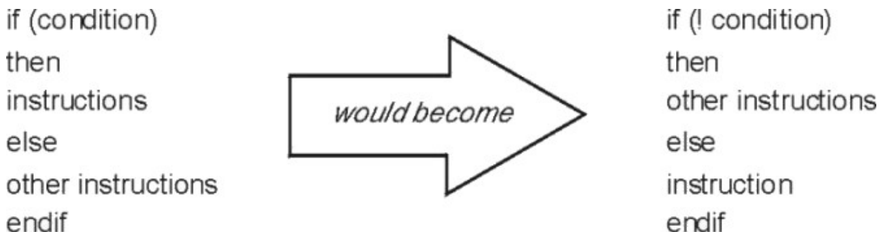
Figure 16. Example of Conditional Branch Recoding
