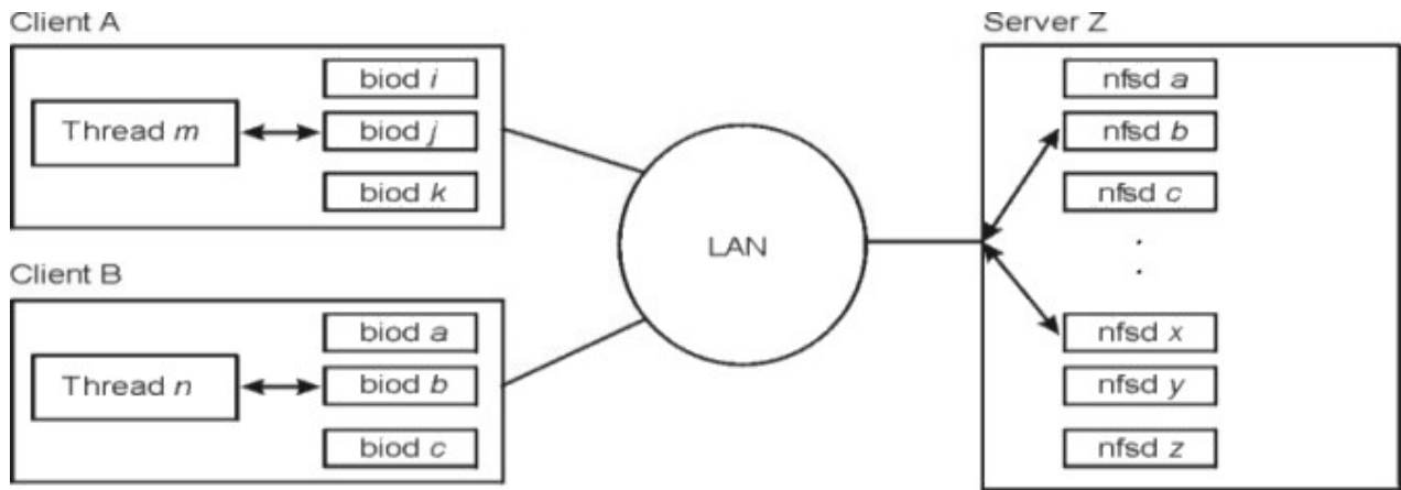
Figure 22. NFS Client-Server Interaction
