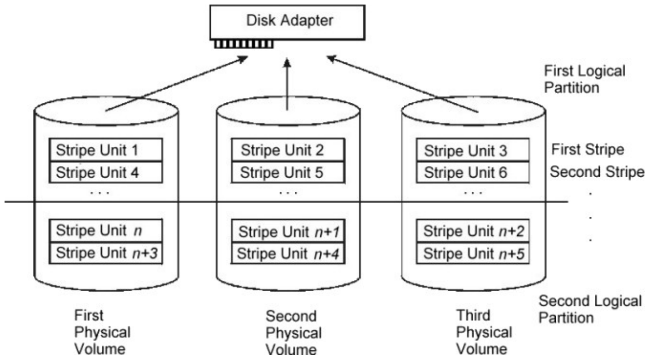
Figure 19. Striped Logical Volume /dev/lvs0
