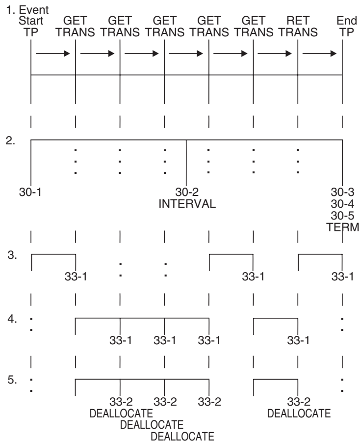
Figure 30. Example of multi-trans shell processing
