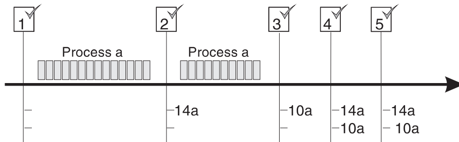
Figure 34. SMF record type 30: Example 2
