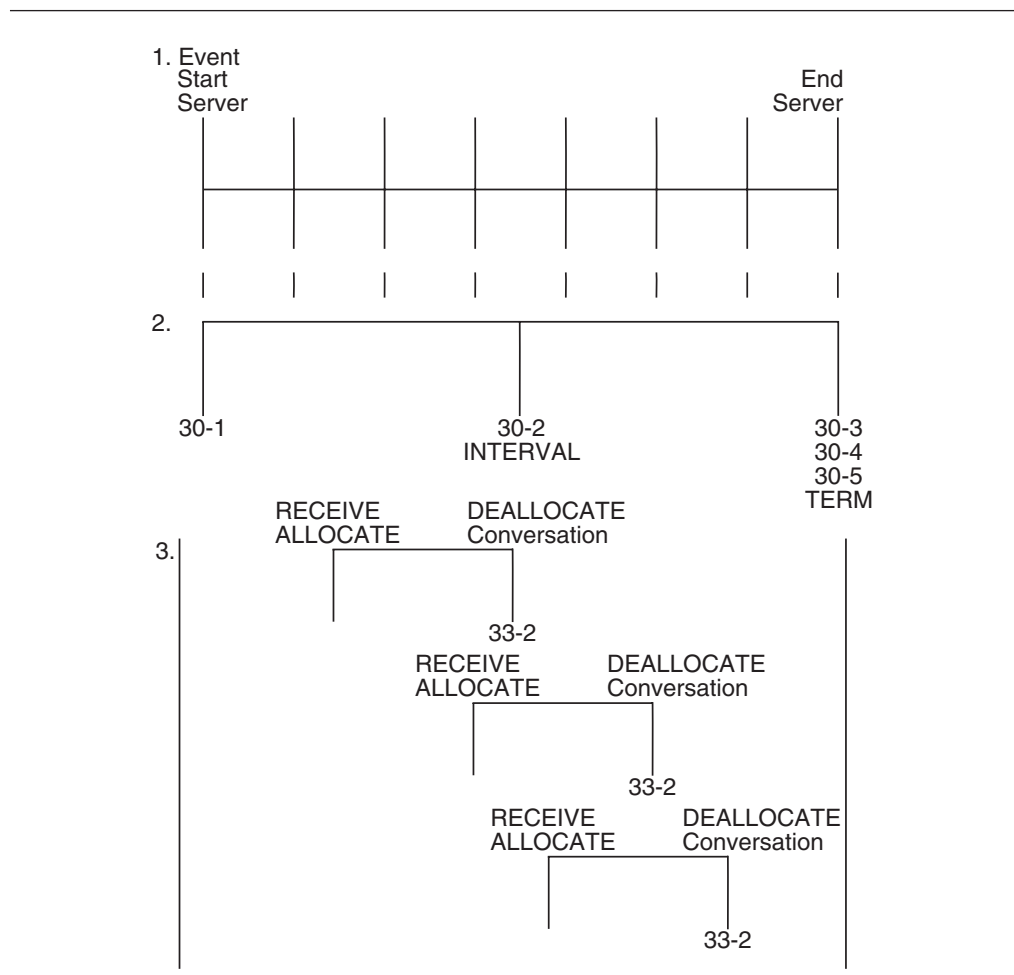
Figure 31. Example of APPC/MVS server processing
