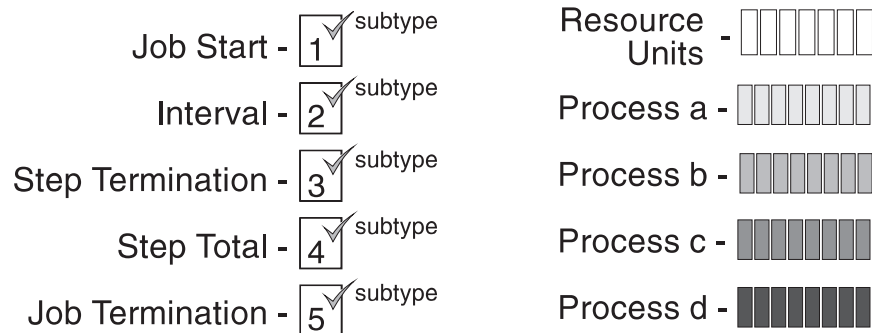
Figure 32. SMF job flow examples - key
