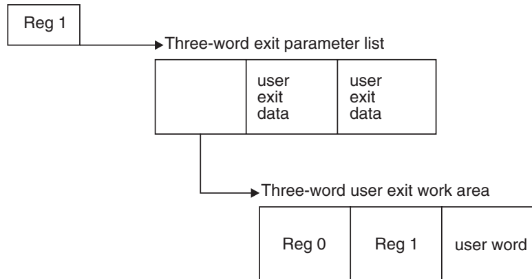
Figure 24. SMF Dump Program Input Parameter Structure
