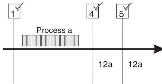
Figure 33. SMF record type 30: Example 1
