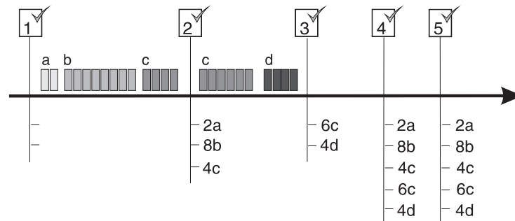
Figure 35. SMF record type 30: Example 3
