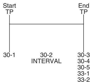
Figure 29. Example of standard TP processing
