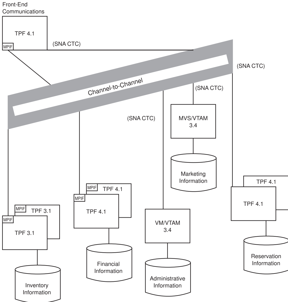
Figure 9. Connecting Configurations Using The MPIF Feature and SNA CTC
