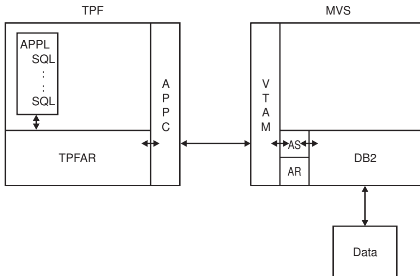
Figure 10. SQL Request Using the TPFAR Feature
