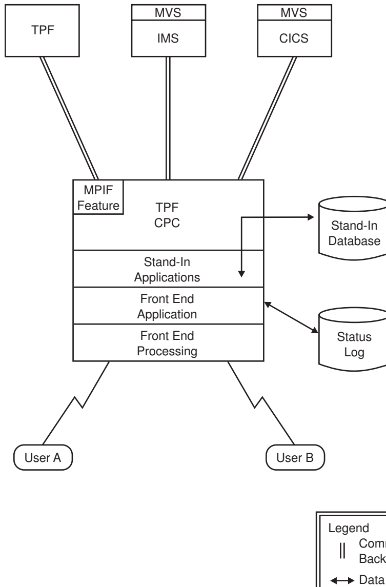
Figure 5. Front-End Processor Application
