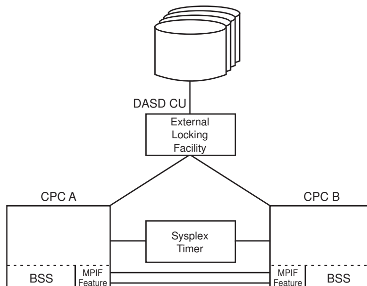
Figure 8. Loosely Coupled Configuration
