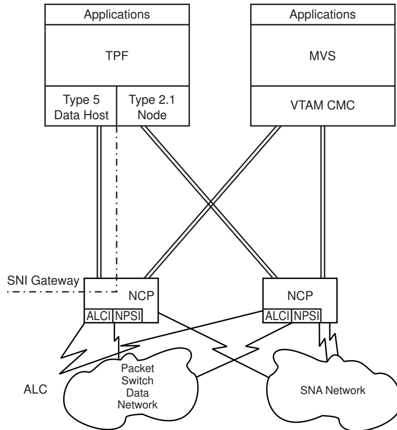
Figure 11. TPF Communication Support
